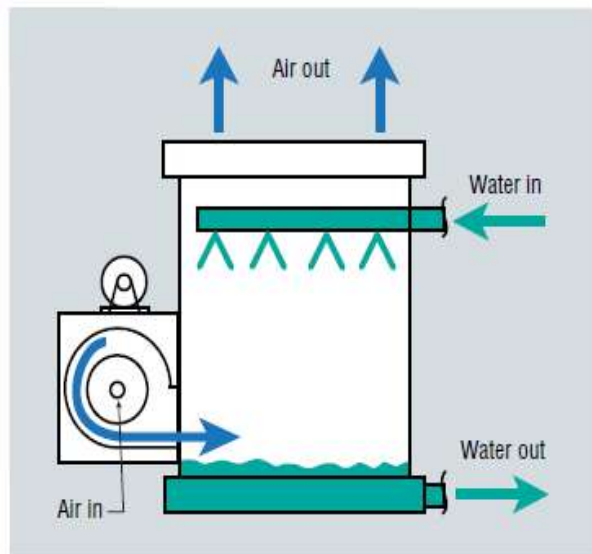
FIGURE 1. A mechanical forced-draft cooling tower.
