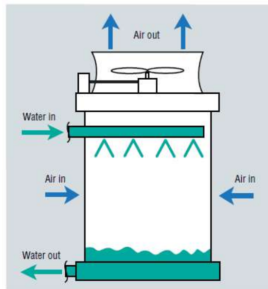
FIGURE 2. A mechanical induced-draft cooling tower.
